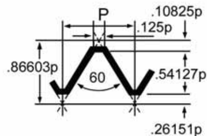
I.S.O. METRIC
