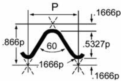
B.S. CYCLE
